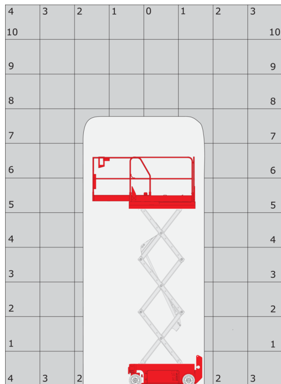
Laaddiagram
